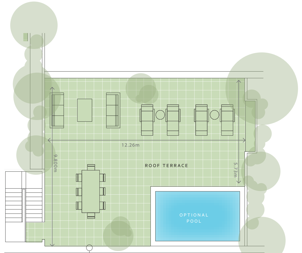
OCEAN CLUB VIEW ROOF LEVEL
